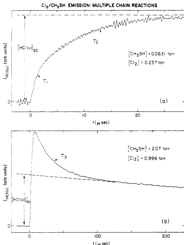
Figure 4. Detailed time-resolved signals of HCl(v = 1) fluorescence from the Cl_2/CH_3SH chain reaction.
