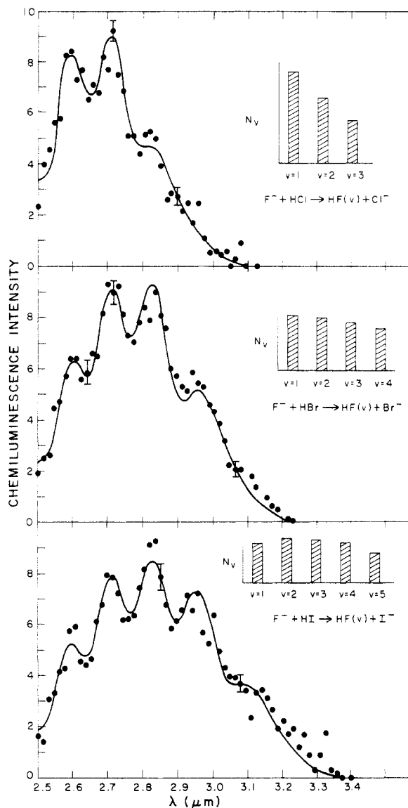
Figure 6. Low-resolution \text{HF}(v) spectra and their best fit vibrational distributions after radiative cascade corrections for the \text{F}^- + \text{HX} \rightarrow \text{HF}(v) + \text{X}^- reactions.
