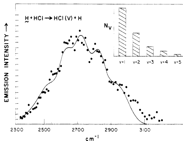
Figure 5. Early time low-resolution HCl(v) spectrum from the T-V excitation of HCl by translationally fast H atoms ( H ). The spectrum includes the contributions of various v \rightarrow v - 1 bands, which are anharmonically shifted to longer wavelengths. The inset shows the vibrational distribution of the best fit.
